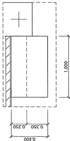
PLAN VIEW SCALE 1 : 12.5
