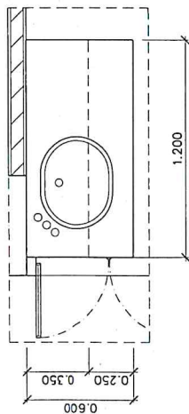
PLAN VIEW SCALE 1:12.5
